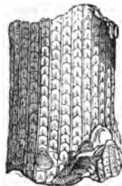
FAVULARIA TESSELLATA. (One-fifth nat. size.)
